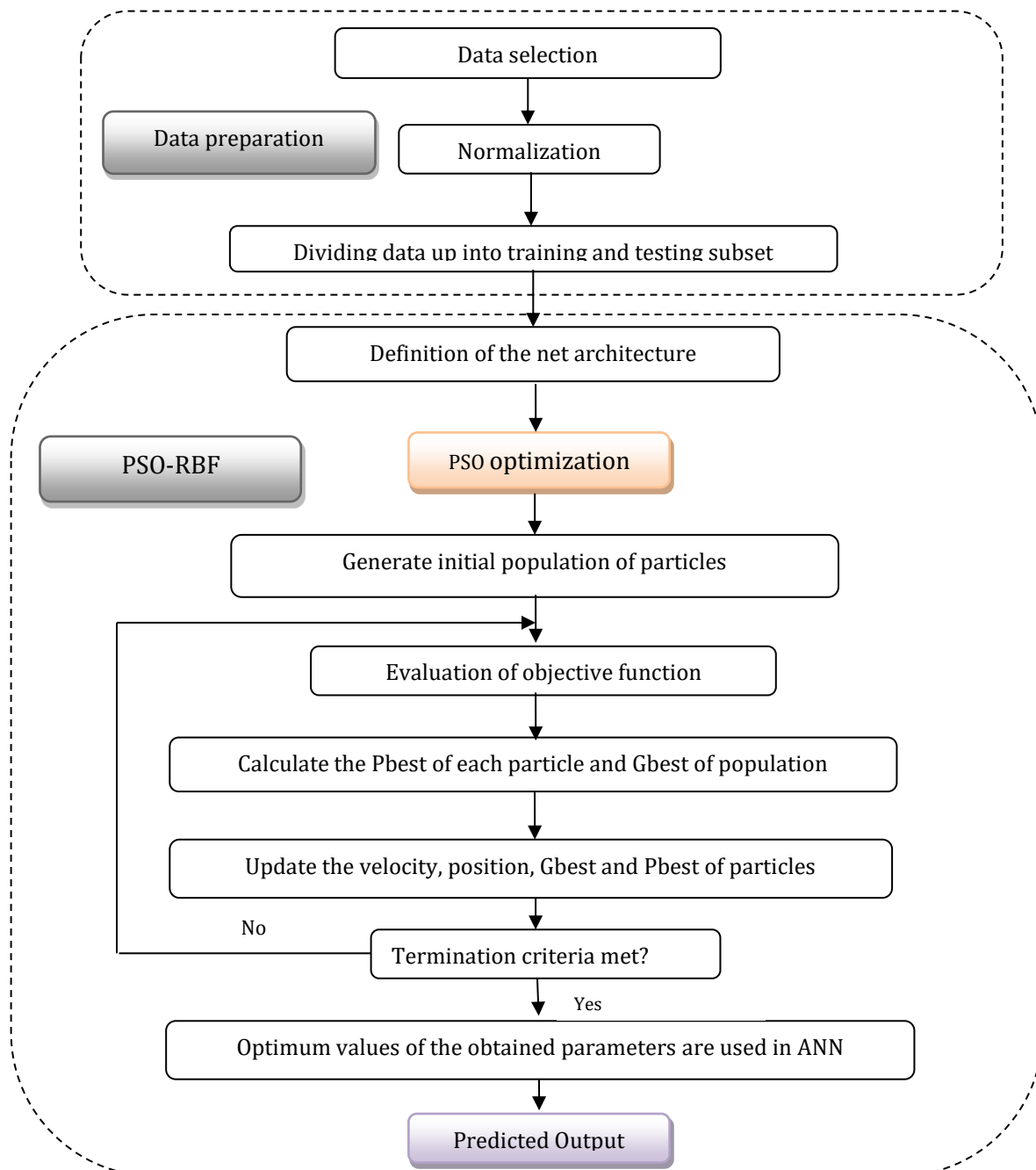
Fig. 2. presents the flowchart of the suggested RBF-PSO algorithm.
