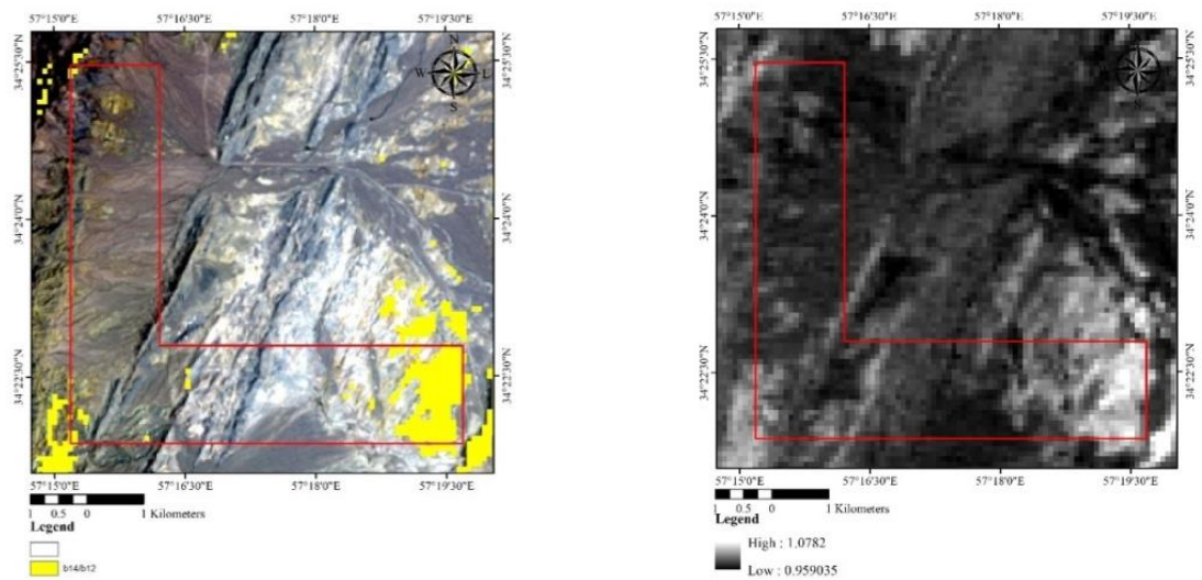
Fig. 15. Band ratio 14/12 of ASTER satellite imagery for the identification of areas containing quartz
