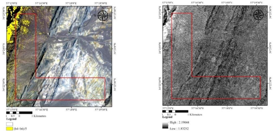
Fig. 14. Band ratio (4+6)/5 of ASTER satellite imagery for the identification of areas containing alunite and kaolinite
