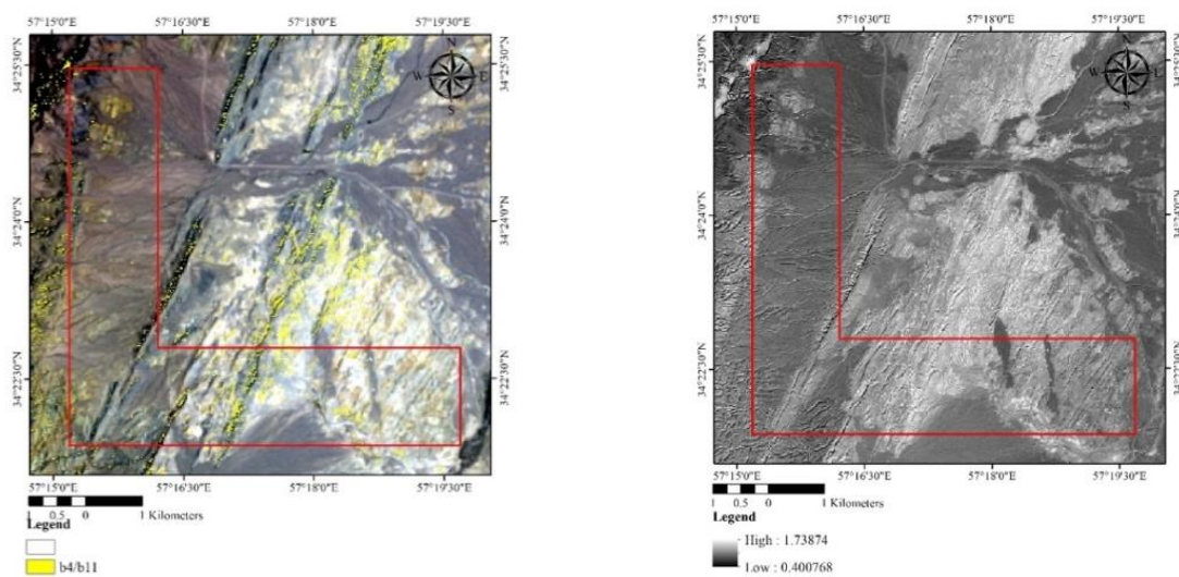
Fig. 19. Band ratio 4/11 of Sentinel satellite imagery for identifying areas containing ferrous iron oxide ( \text{Fe}^{2+} )
