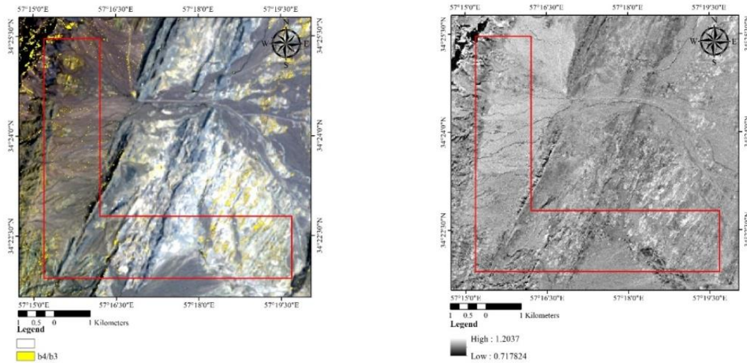
Fig. 17. Band ratio 4/3 of Sentinel satellite imagery for the identification of areas containing iron oxides
