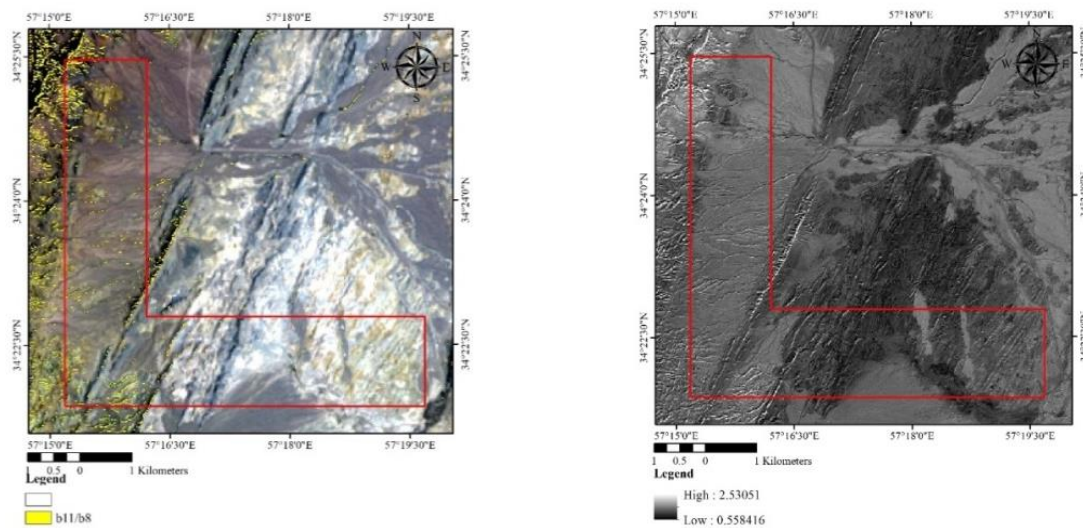
Fig. 18. Band ratio 11/8 of Sentinel satellite imagery for the identification of areas containing ferric iron oxide ( \text{Fe}^{3+} )
