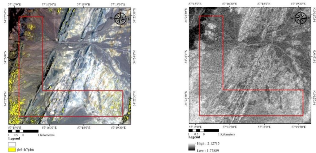
Fig. 13. Band ratio (5+7)/6 of ASTER satellite imagery for the identification of areas containing muscovite, illite, and smectite
